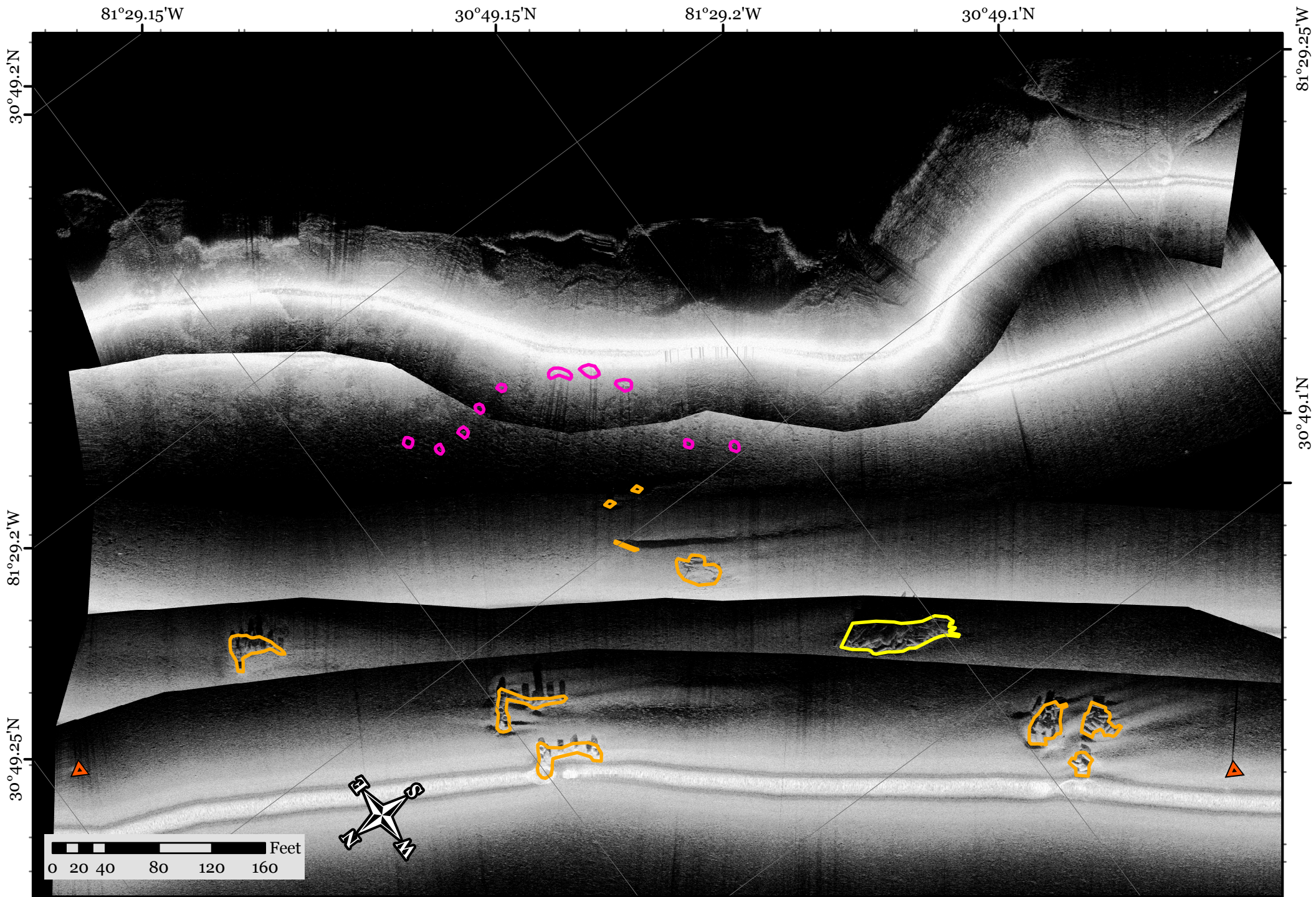
Map of existing structures at Stafford Island inshore artificial reef with side scan sonar imagery taken at high tide on June 26th, 2018.
