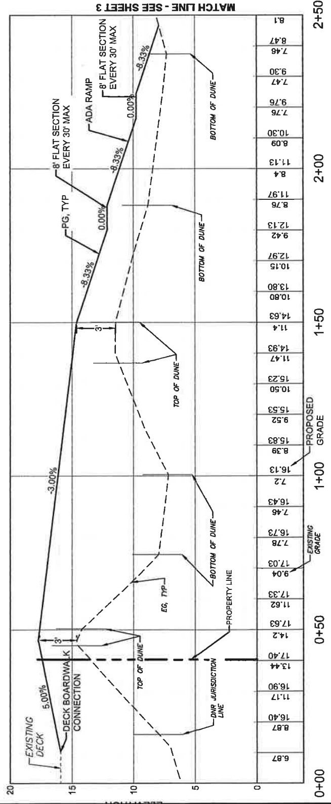
BOARDWALK ELEVATION PROFILE SCALE: 1" = 20' HORIZ. 1" = 5' VERT.
