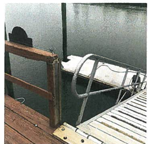
Photo 6: Existing ramp and floating dock
