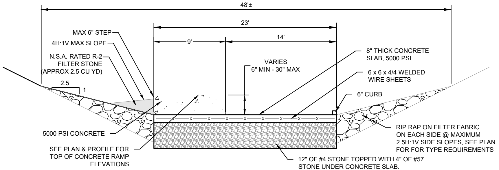
TYPICAL SECTION @ CONCRETE DOCK RAMP NO SCALE
