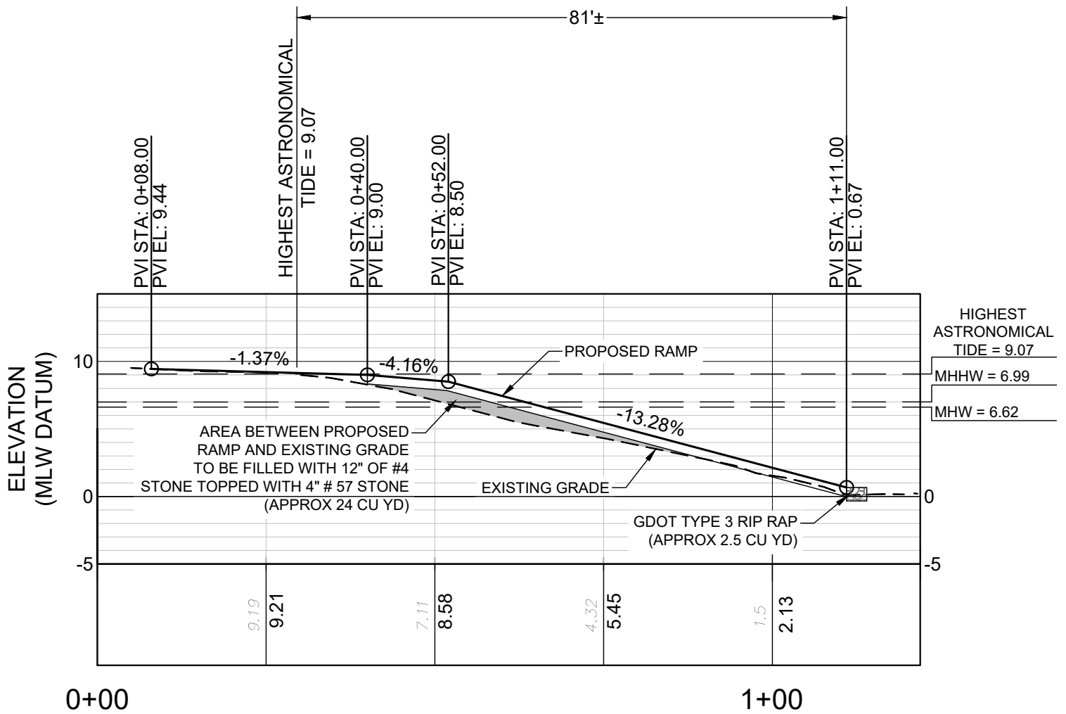
BOAT RAMP PROFILE HORZ SCALE: 1" = 20' VERT SCALE: 1" = 10'
