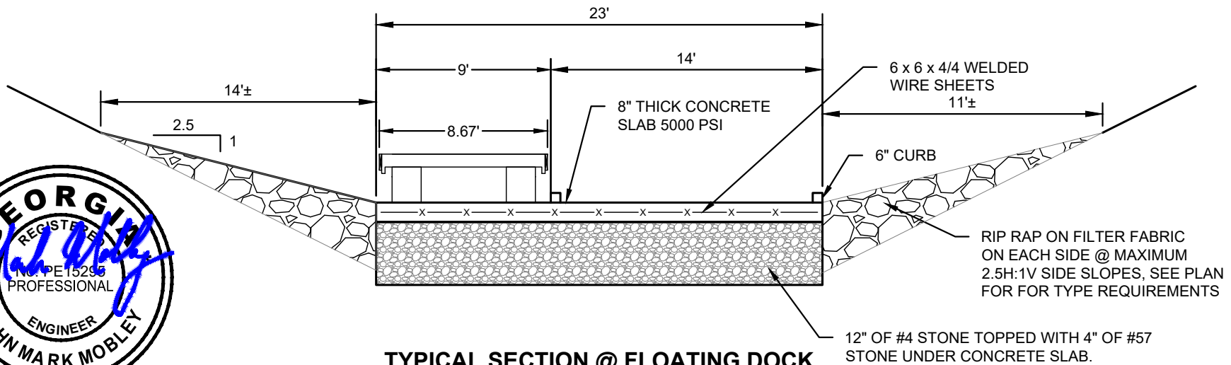
TYPICAL SECTION @ FLOATING DOCK NO SCALE
