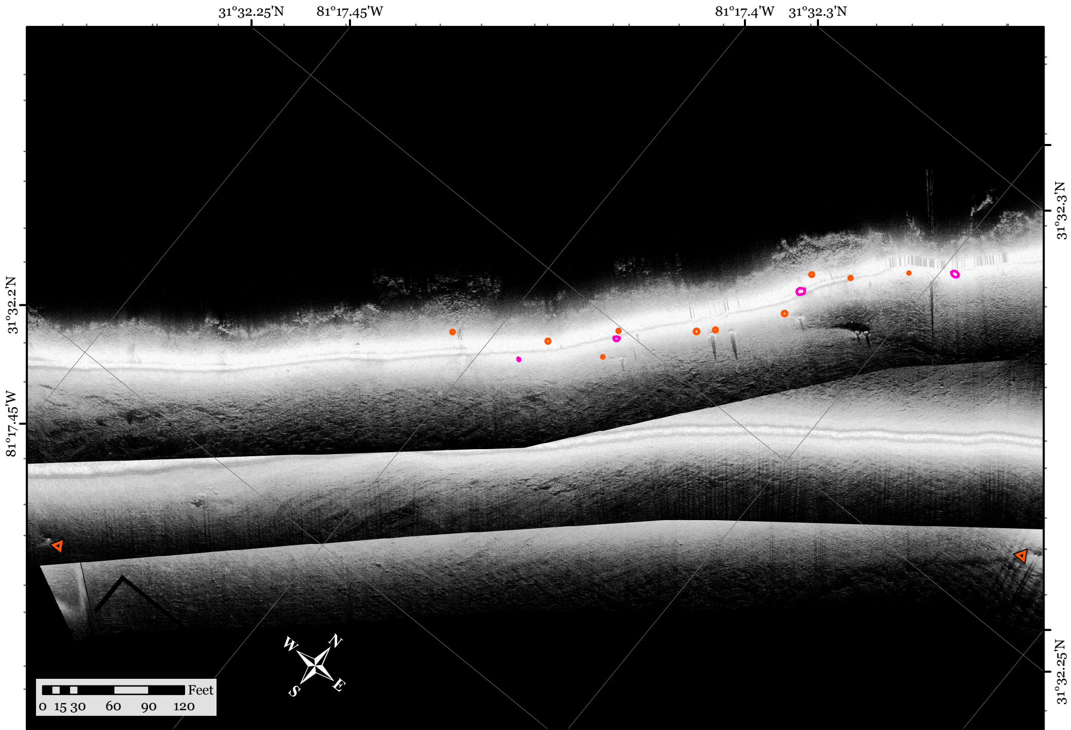
Map of existing structures at Four Mile Island inshore artificial reef with side scan sonar imagery taken at high tide on June 25th, 2018.
