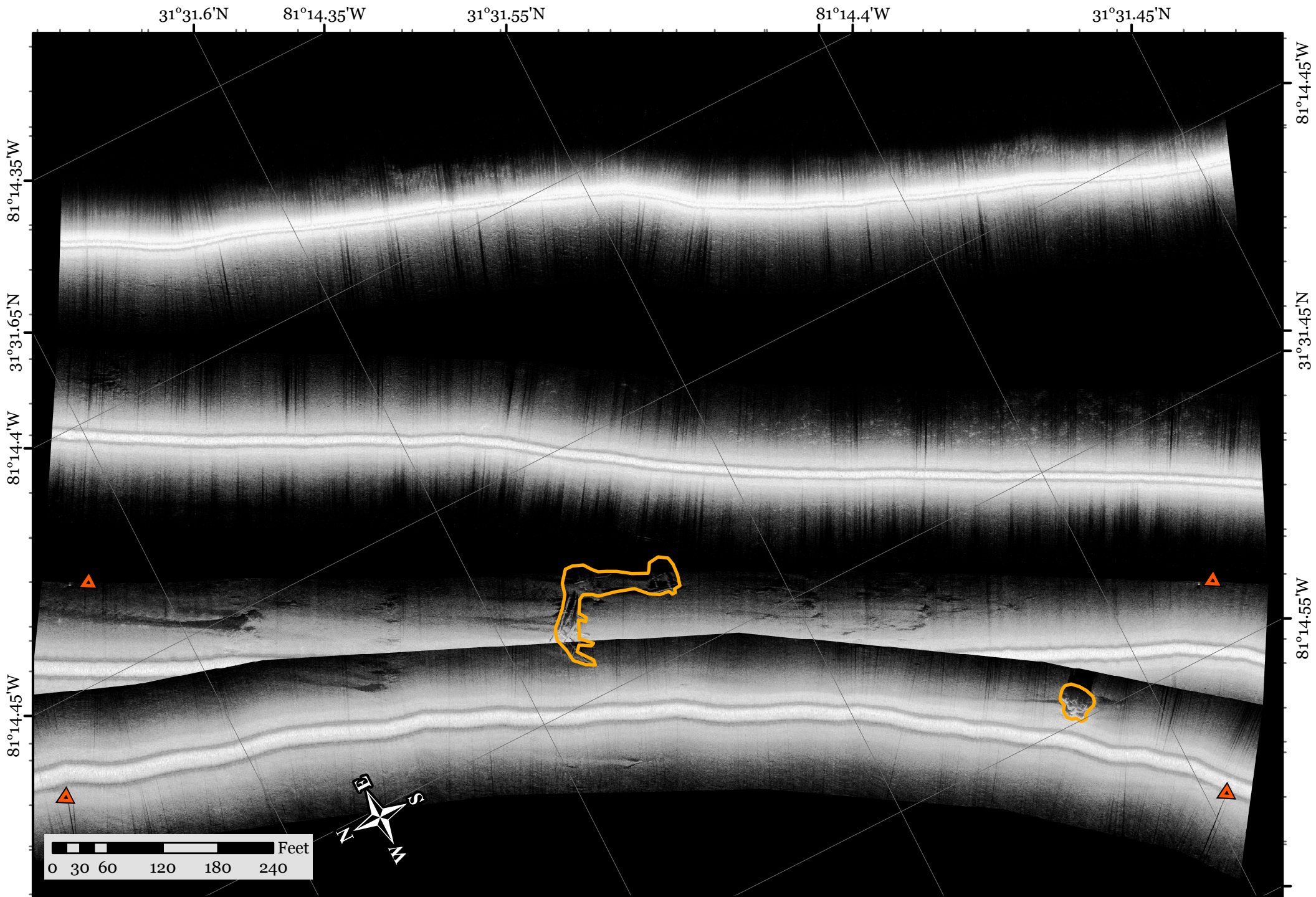
Map of existing structures at High Point inshore artificial reef with side scan sonar imagery taken at high tide on June 25th, 2018.
